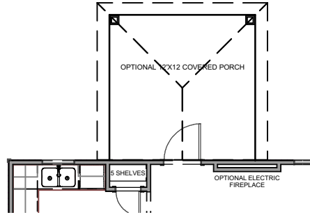
OPTIONAL COVERED PORCH
