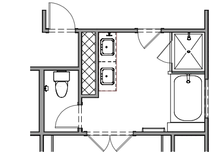
MASTER BATH OPTION 1- 42" ACRYLIC TUB & 48"x42" TILE SHOWER
