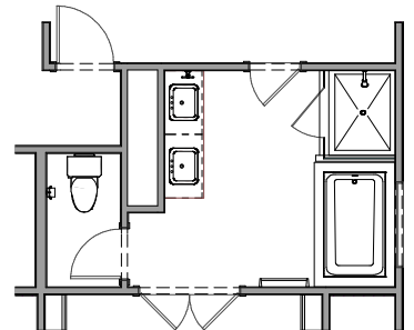
MASTER BATH OPTION 3- RECTANGLE DROP-IN TUB & 48"x42" TILE SHOWER
